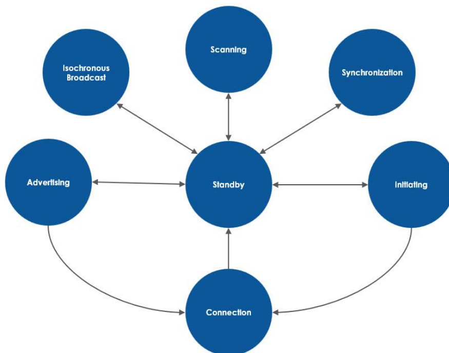
Figure 2 The Link Layer state machine
